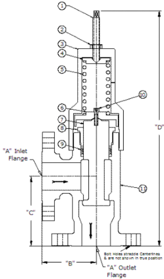
Model PRH-04-1500#Fig 1500# ANSI Flanged connections
